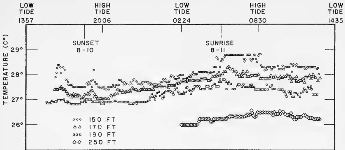
Figure 3. Temperature records for the first day, Buoy 5, at various depths.
